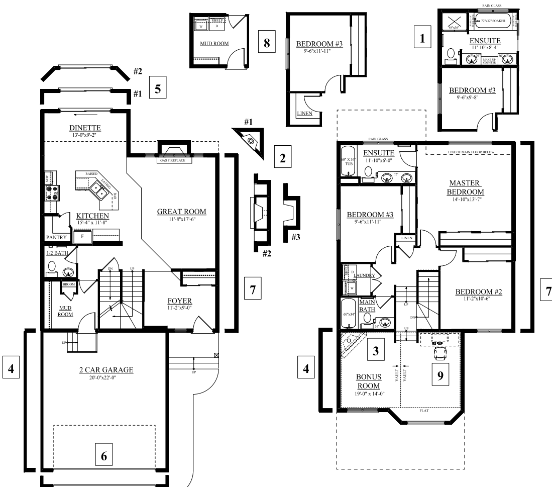
SECOND FLOOR PLAN 1050 SQ.FT.
