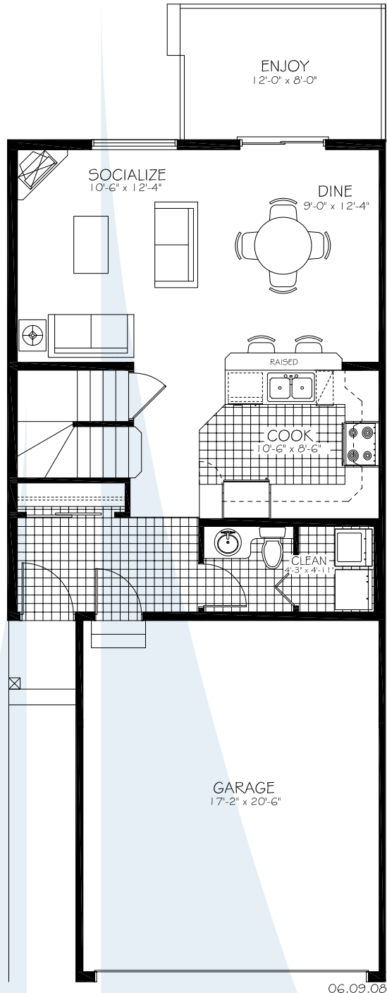
MAIN FLOOR • 613 SQ. FT
