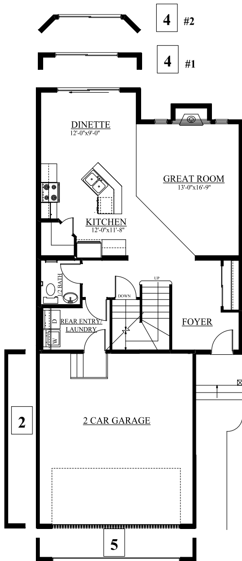
MAIN FLOOR PLAN 829 SQFT
