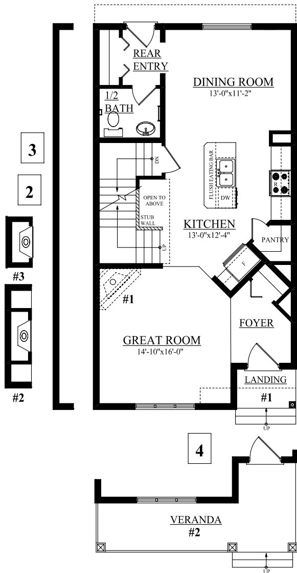
MAIN FLOOR 736 SQ.FT.
