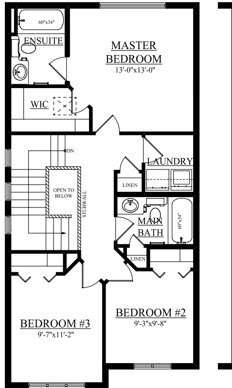
SECOND FLOOR 702 SQ.FT.
