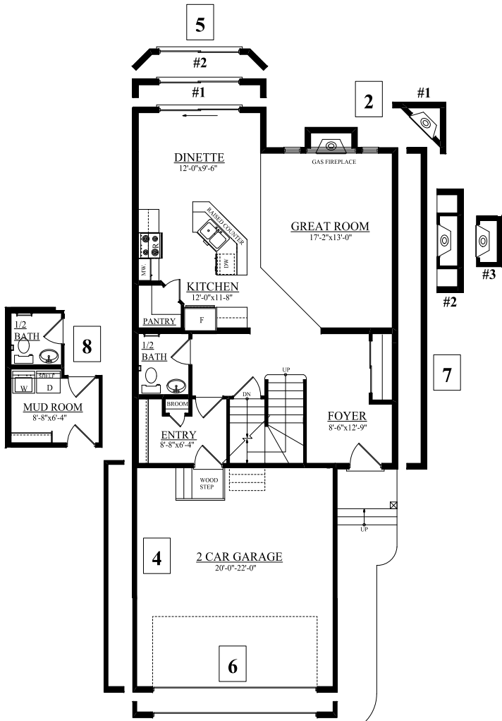
MAIN FLOOR 881 SQFT
