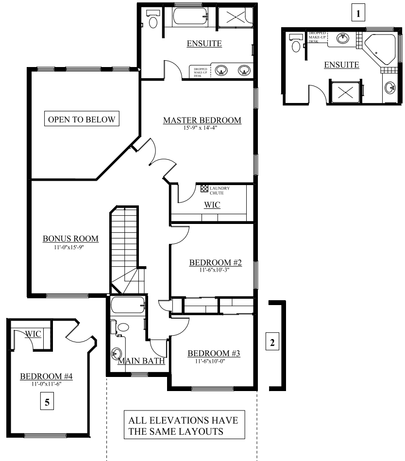
SECOND FLOOR PLAN 1176 SQFT
