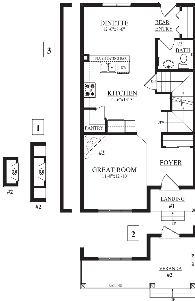
MAIN FLOOR 683 SQ.FT.
