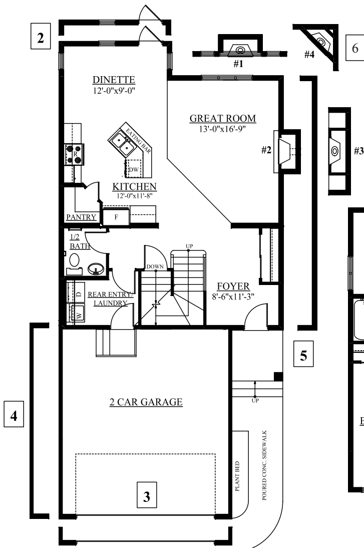
MAIN FLOOR 829 SQ FT
